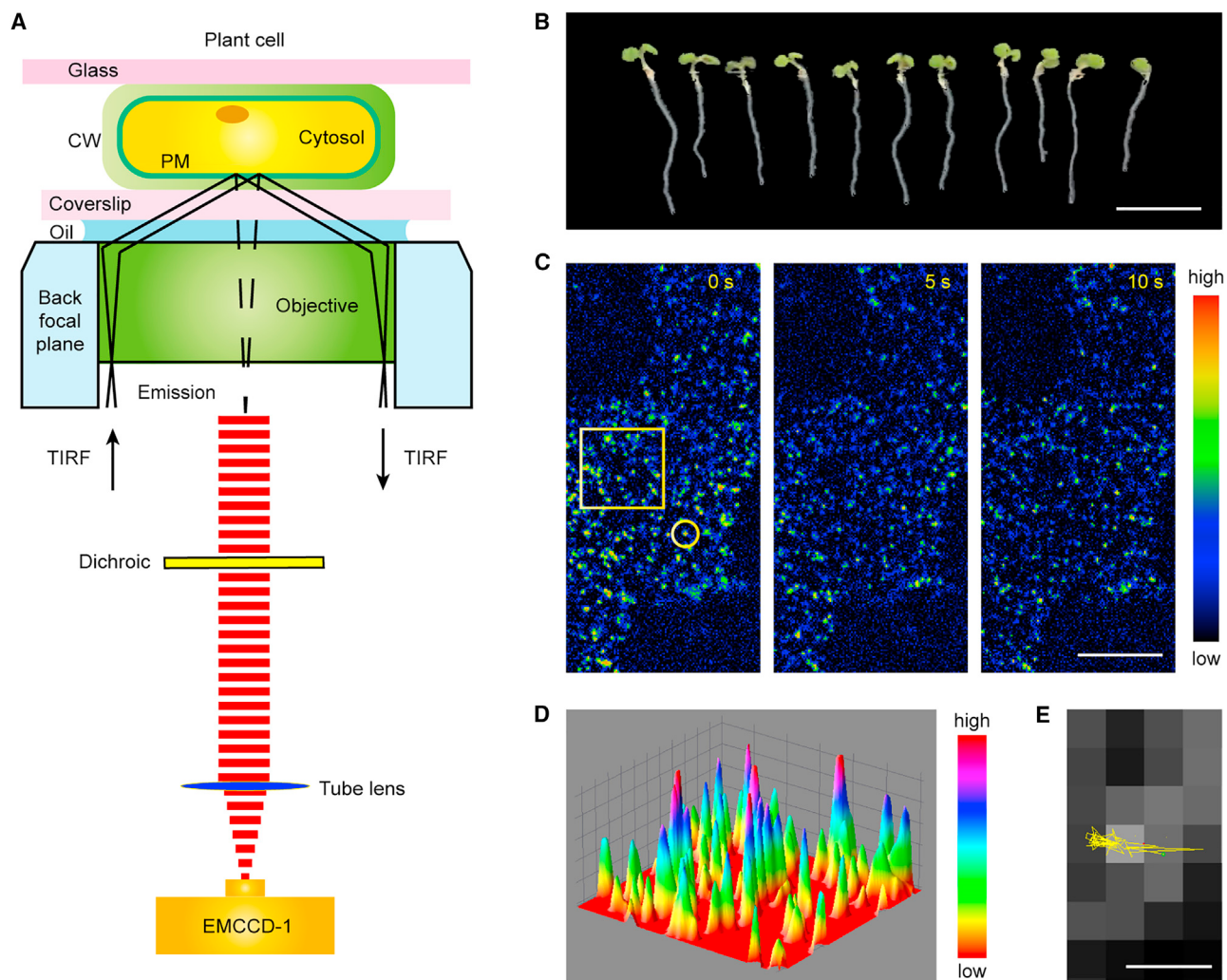
Figure 1. Detection of a GFP-Tagged Protein in Arabidopsis thaliana .
