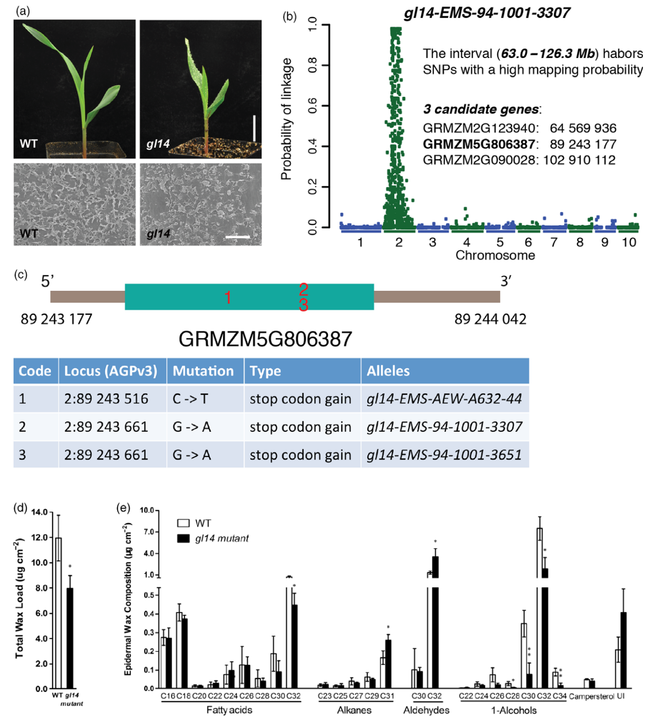
Figure 5. gl14 cloning. (a) Phenotype of the gl14 mutant (the gl14-EMS-94-1001-3307 homozygous mutant) and wildtype after water spraying (bar = 3 cm) and SEM photographs ( \times 10\,000 magnification, bar = 3 \mu\text{m} ). (b) BSR-Seq to map the gl14 gene using the mutant allele of gl14-EMS-94-1001-3307 . The mapping interval was based on SNPs showing a high probability ( >0.975 ) of complete linkage between the SNP and the gl14 gene. Candidate genes are the genes harboring at least one large-effect variant in EMS mutants and in the turquoise co-expression module. (c) The candidate gene, GRMZM5G806387, was confirmed to be the gl14 gene by showing that three alleles from at least two independent EMS mutagenesis events carried EMS-type mutations, all of which introduce premature stop codons, and presumably caused the encoded truncated proteins. (d, e). Total epicuticular wax loads, wax component analysis and comparison in gl14 mutants (the gl14-EMS-94-1001-3307 homozygous mutant) and wildtype. Values are means of three biological replicates \pm SD. UI indicates unidentified and asterisks indicate statistically significant differences between wildtype and gl14 mutants ( *P < 0.05 , **P < 0.01 , Student's t -test).
