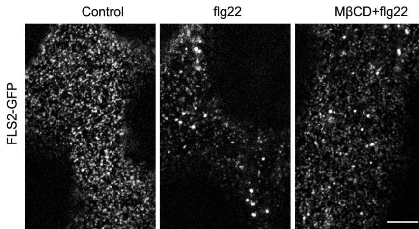
Fig. S6. Typical images showing diffraction-limited fluorescent spots of FLS2-GFP on a fixed cell membrane of Arabidopsis leaf epidermal cells under flg22 treatment and co-treatment with MβCD and flg22, imaged with TIRFM. The image is a section of the first frame of a stack of images with the background subtracted (Scale bar: 1 μm).
