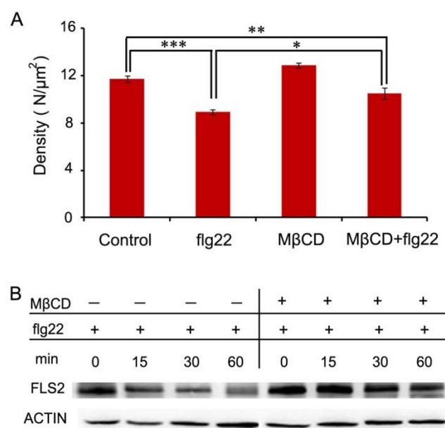
Fig. S11 Sterols are involved in flg22-induced FLS2 degradation.
