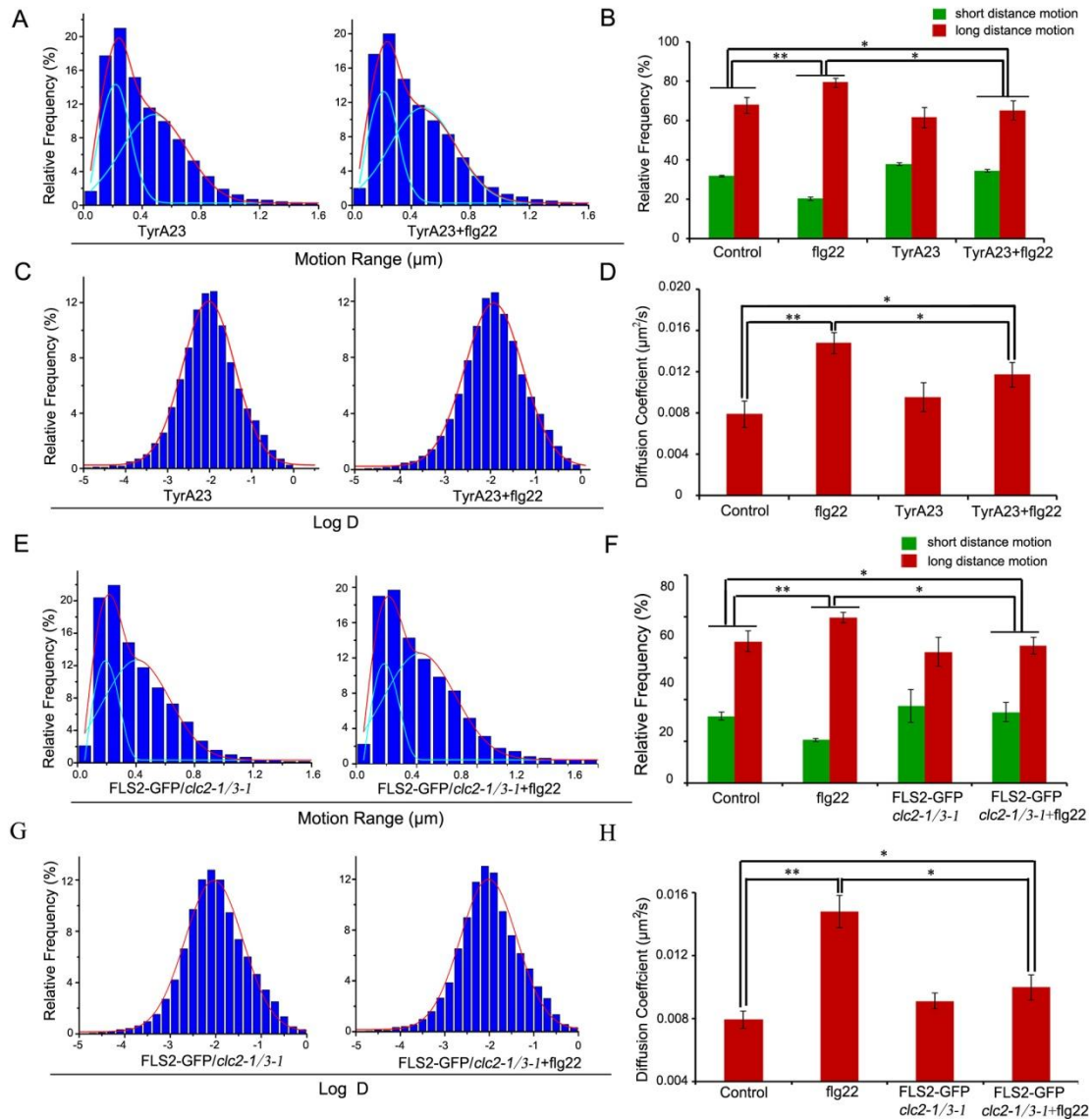
Fig. S7. Clathrin is required for FLS2 dynamics.
