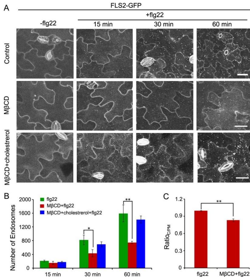
Fig. S10. Sterols are involved in flg22 induced FLS2 endocytosis.
